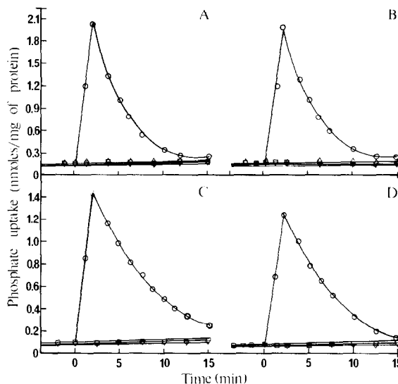
Fig.2. Transient uptake of P_i into membrane vesicles of P. denitrificans driven by the addition of salts. P_i uptake into right-side out (A,C) and inside out (B,D) vesicles was measured in a 2ml incubation mixture which contained: 1 \mu mol [ ^{32} P] P_i (0.25 \mu Ci/ \mu mol), 0.2 ml of the vesicle suspension (1.5 mg protein) and 100 \mu mol Tris-Cl (pH 7.3). At time 0 min either 150 mM KCl (A,B) or 150 mM NH_4 Cl (C,D) were added. In A and B 1 \mu g nigericin was included in the incubation mixture. Further additions and subtractions to the incubation mixture were made as follows: none (○), plus 5 \mu M FCCP (●), minus nigericin (△), plus 1 \mu g valinomycin, minus nigericin (▽).
