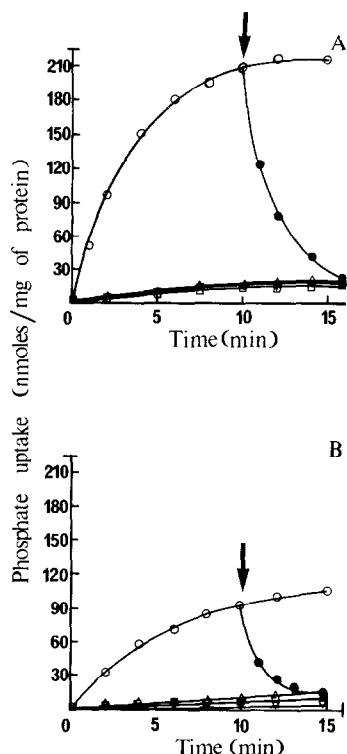
Fig.1. Respiration-driven P_i uptake in membrane vesicles of P. denitrificans . P_i uptake into right-side out (○, ●, △) and inside out (△, ▽) vesicles was measured in a 2 ml incubation mixture which contained: 1 \mu mol [ ^{32} P] P_i (0.25 \mu Ci/ \mu mol), 0.2 ml of the vesicle suspension (1.5 mg protein), 100 \mu mol Tris-Cl (pH 7.3) and either 20 mM sodium ascorbate plus 0.1 mM PMS (A), or 10 mM sodium succinate (B). FCCP (5 \mu M) was either omitted (○, △) included in the incubation mixture (●, ▽), or added at time 10 min (●).
